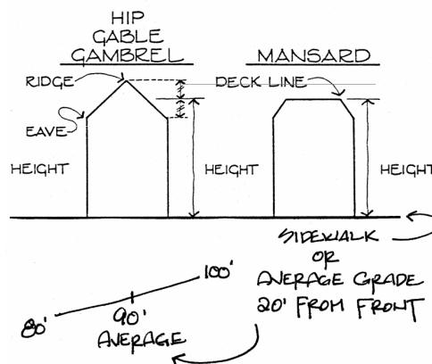
FIGURE 10-2 BUILDING HEIGHT
